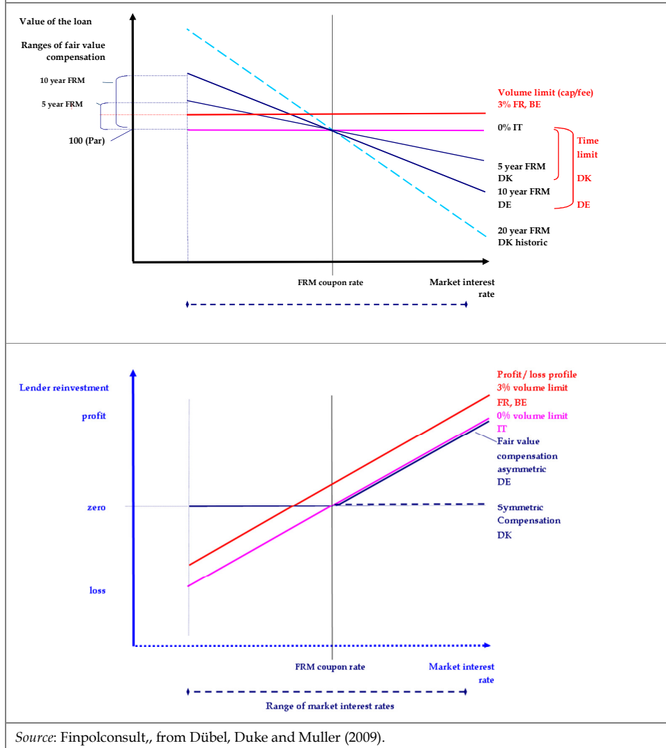
Figure 14. Conceptual framework for the pricing of non-callable FRM
